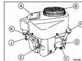
Parts Location
